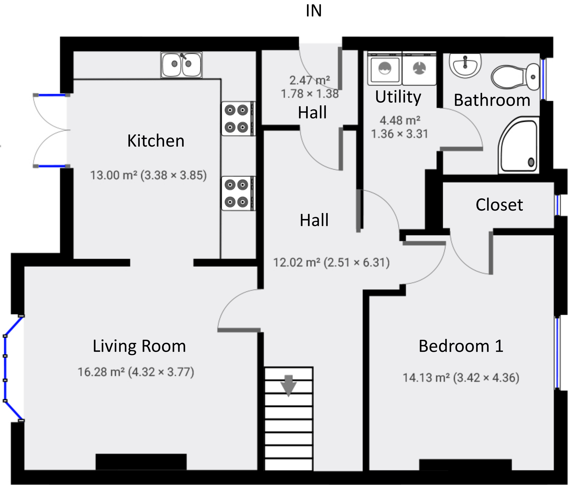
Ground Floor
