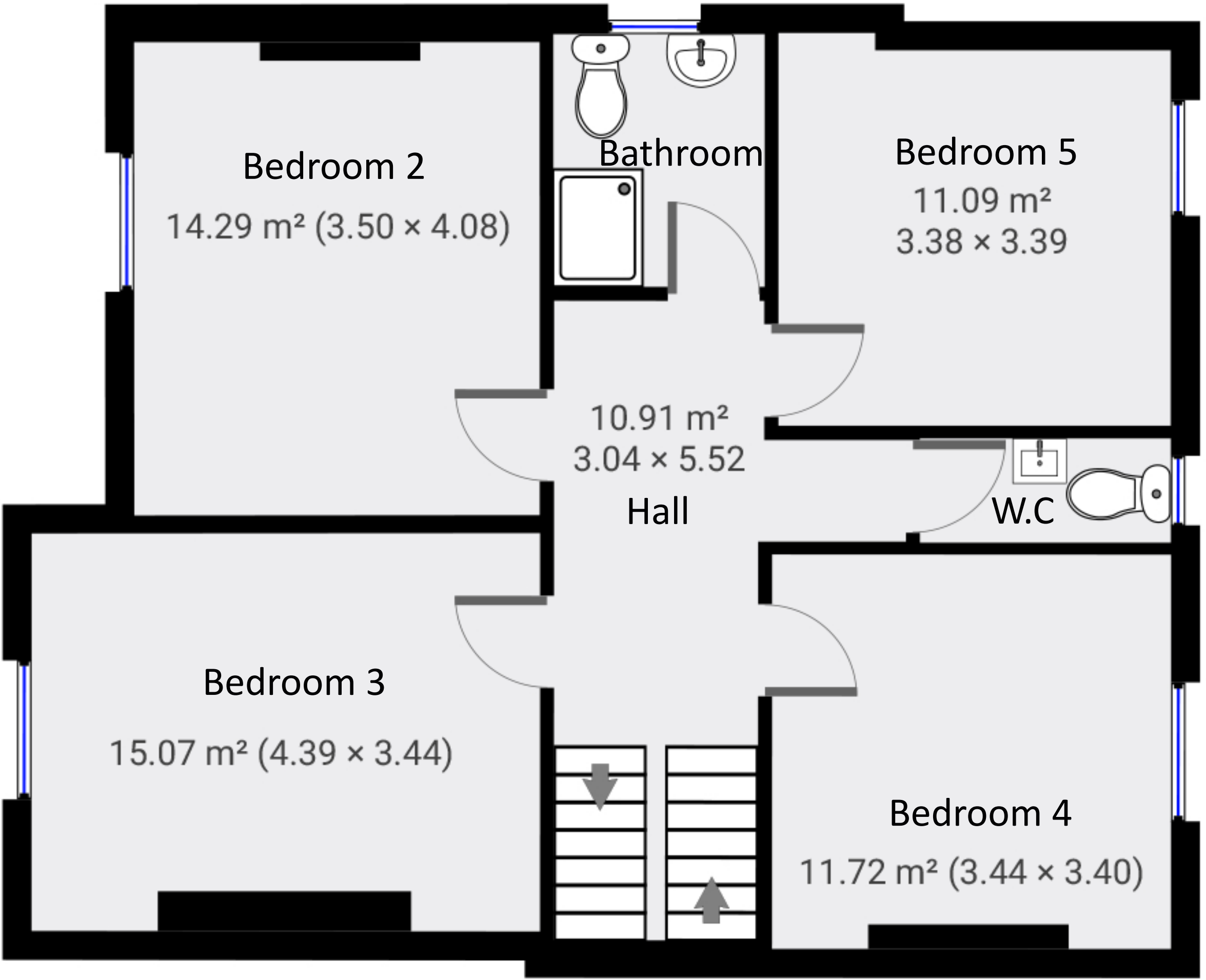
1st Floor
