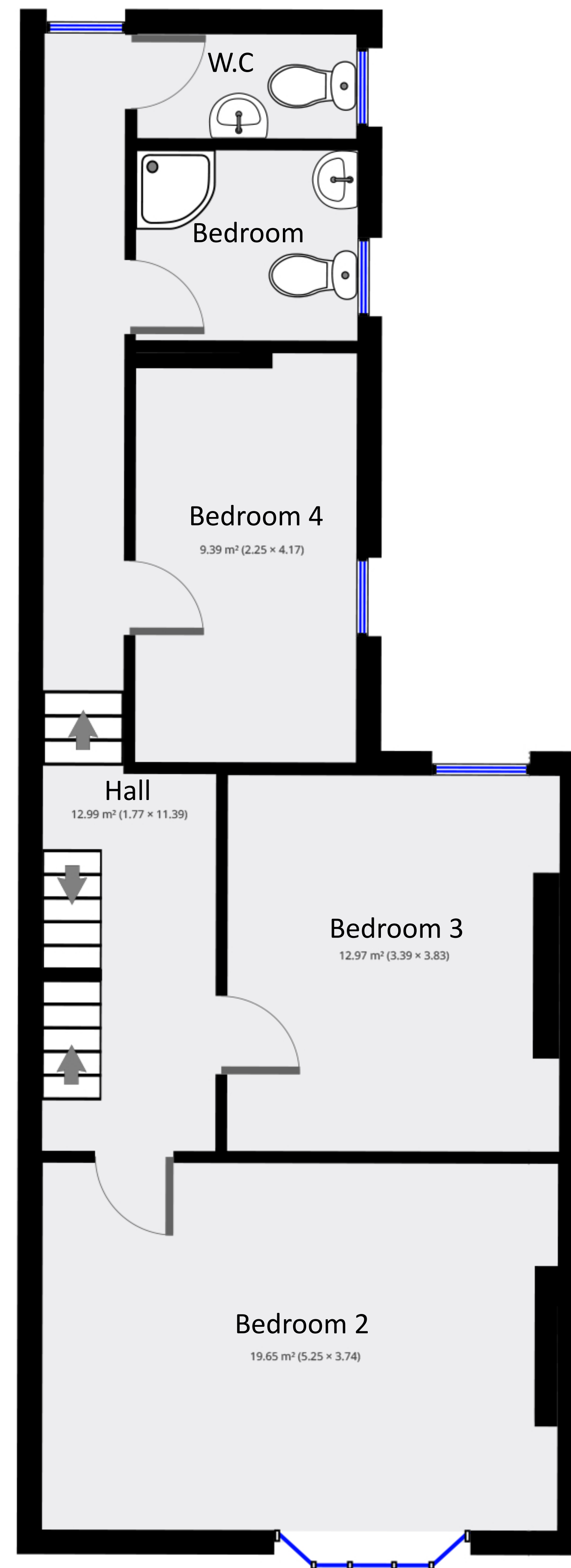
1st Floor
