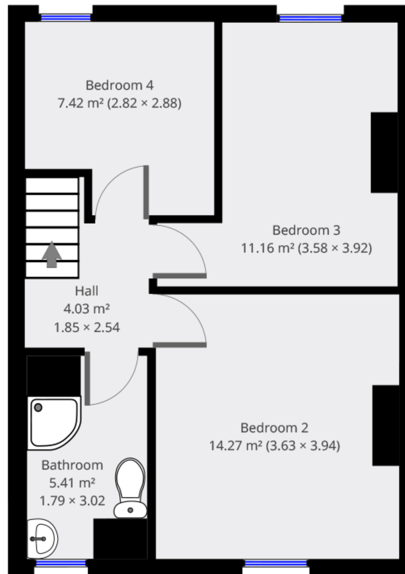
1st Floor
